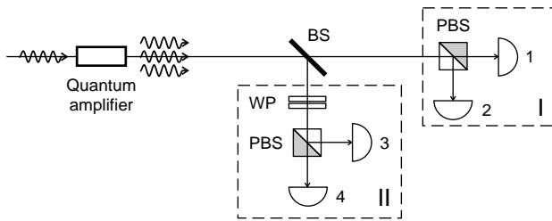
Figure 1 Experimental setup for retrieving information from a single photon. BS are the beamsplitters, PBS are the polarizing beamsplitters, WP is a waveplate to switch between vertical/horizontal and \pm 45^\circ polarizations, and 1–4 are the photodetectors. Part I of the experimental setup measures vertical/horizontal polarizations, whereas part II – \pm 45^\circ polarizations
